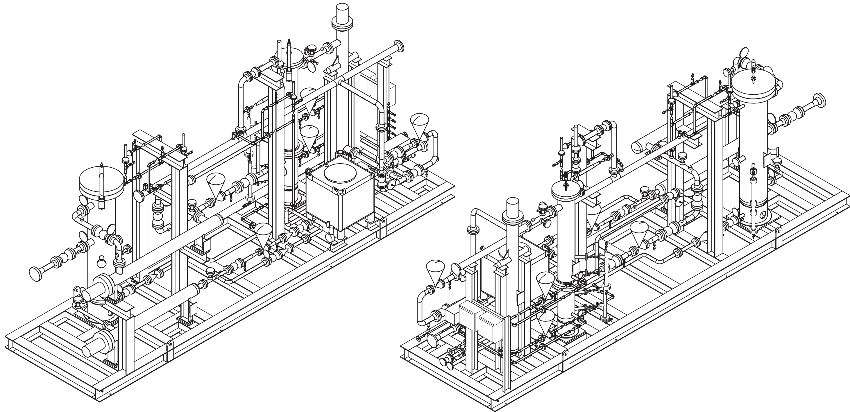
ISO VIEWS (FOR REFERENCE ONLY)
